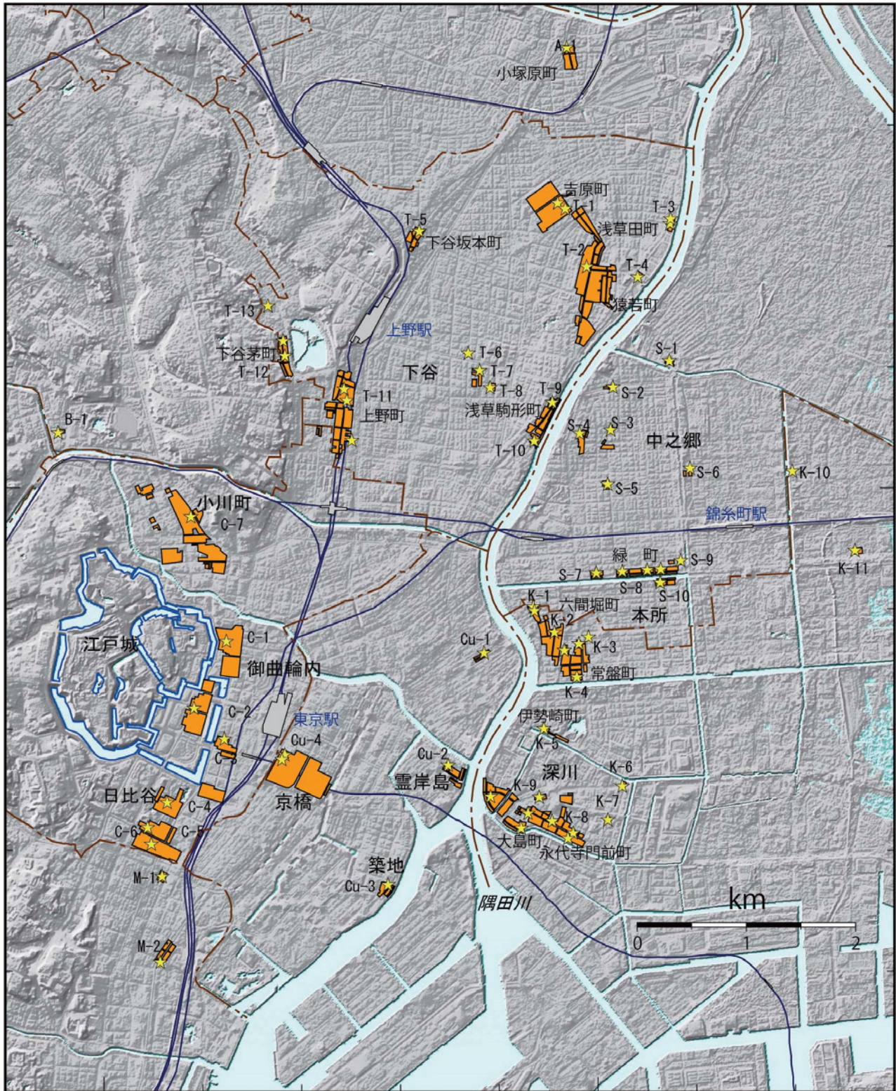
図1. 江戸市中の地震火災の焼失図(橙色)と出火点(黄色星印). [中村・他(2005)に加筆]. 背景の現代の陰影起伏図には区境(茶破線), JR 東日本の路線(青線)と主な駅(灰色多角形)も示した. Fig. 1. Map of burned areas (orange) and locations of fire origins (yellow stars) in Edo city after the earthquake. The ward-boundaries (brown single dotted lines), JR East railways (blue lines) and major stations (gray areas) are also shown on the background map of the present elevation topography.
